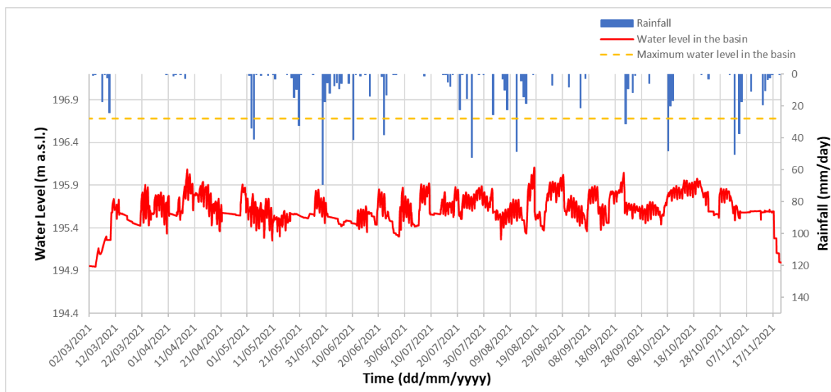
Figure 5.7. Rainfall affecting the Giavenale di Schio area and water level in the basin during the 2021 summer period.
