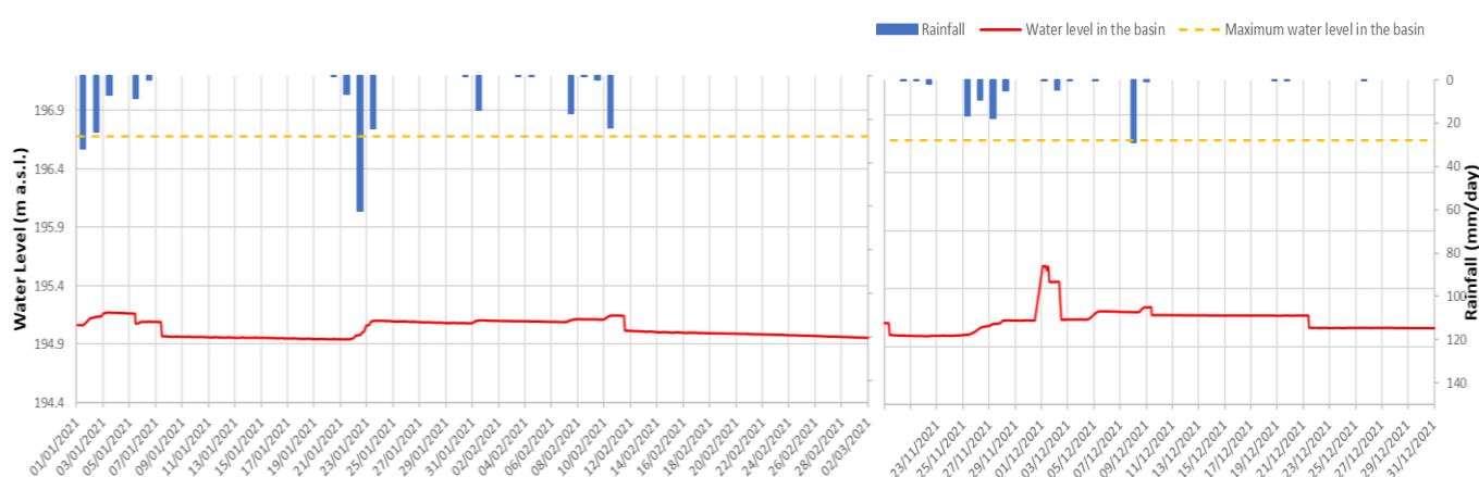
Figure 5.8. Rainfall affecting the Giavenale di Schio area and water level in the basin during the 2021 winter period.
