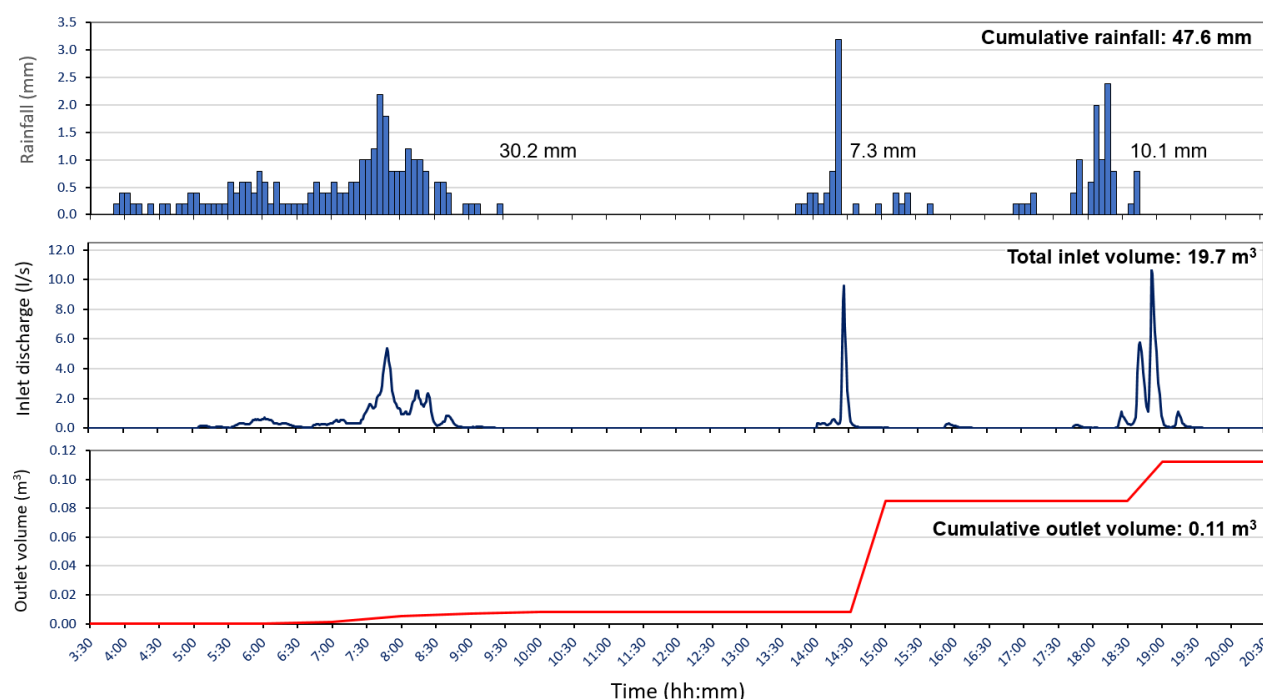
Figure 5.3. Rainfall affecting the urban area of Santorso Municipality the 11 th of May 2020 (first graph), and the consequently measured inlet and outlet runoff from the Intervention 1 of Action C4 (rain garden located in Piazza della Libertà).
