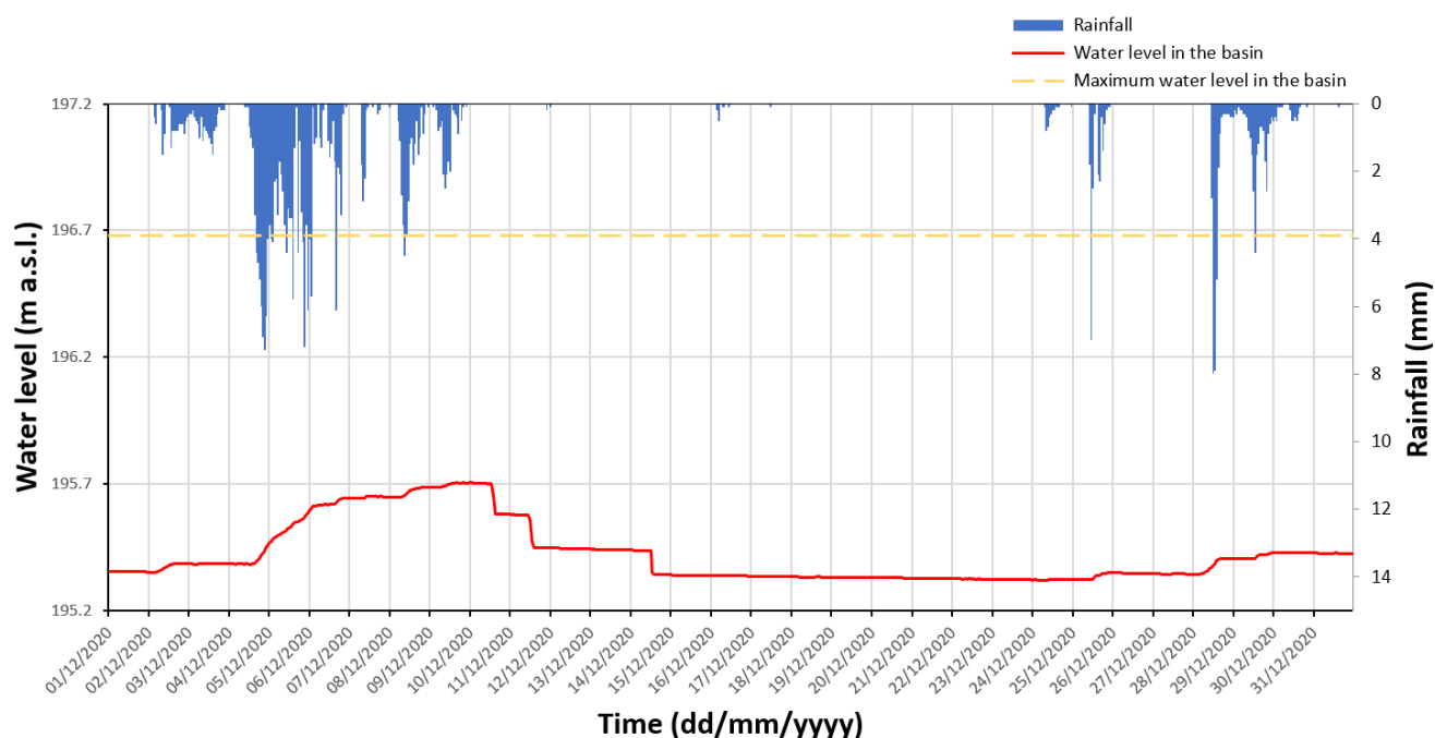
Figure 5.6. Rainfall affecting the Giavenale di Schio area and water level in the basin during the 2020 winter period.
