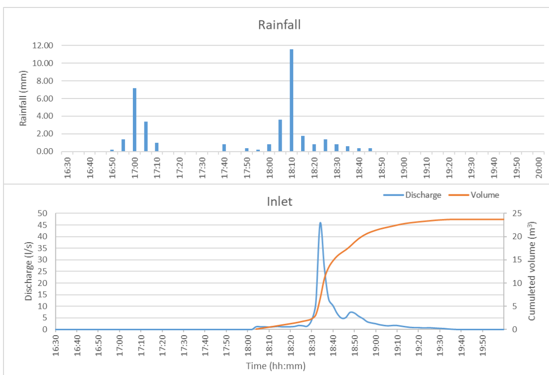
Figure 5.4: Analysis of the rainfall pattern and inlet volume over time of the Piazza della Libertà intervention for the event occurred in 8 th July 2021
